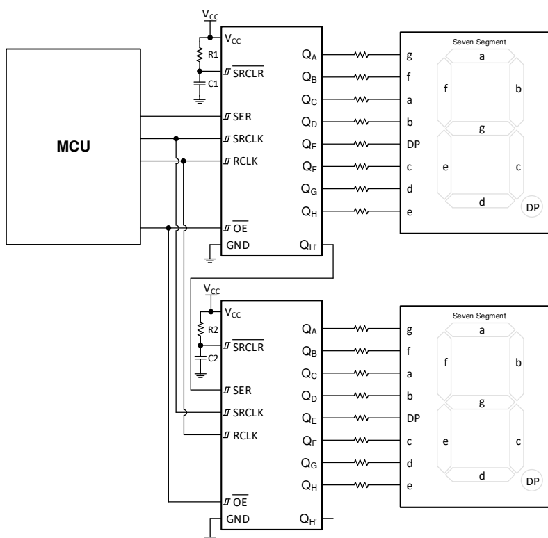
Figure 9-1. Typical application block diagram
